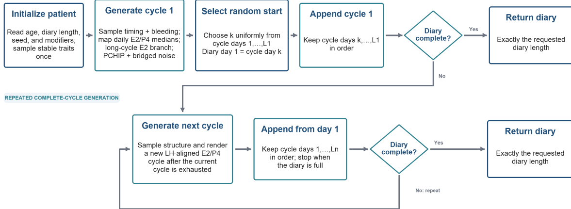
Appendix Figure A1. HORMONE-CYCLE diary-generation workflow. Each generated cycle samples structure and bleeding, maps the LH-aligned daily serum envelope to the realized ovulation and luteal interval, applies the long-follicular E2 branch when applicable, and adds endpoint-bridged serial noise after PCHIP interpolation. Cycle 1 is generated in full and diary day 1 is selected uniformly from its realized cycle days. Output proceeds forward through the remainder of cycle 1 and successive complete cycles until the requested diary length is reached; there is no wrapping.
